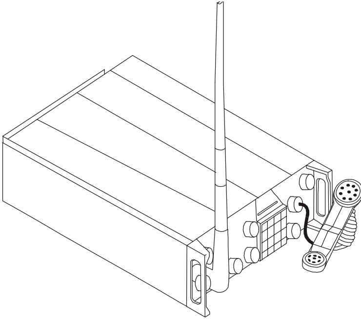
Figure 2-4. AN/PRC-119 SINCARS Radio.
